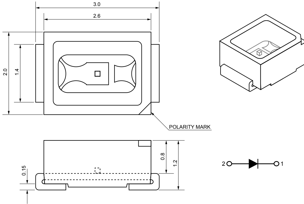
Package Dimensions
